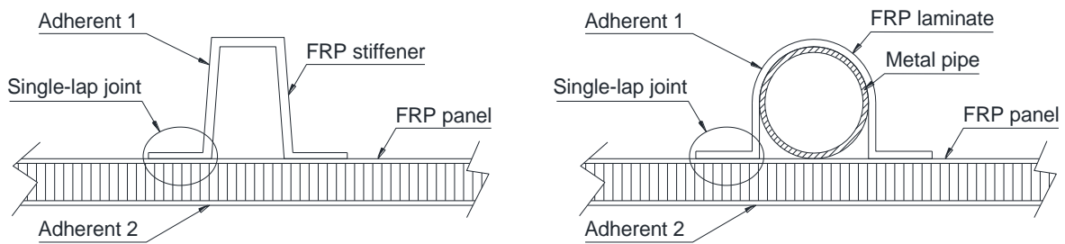
Fig. 1: Adhesive joint between FRP laminate and FRP stiffener
