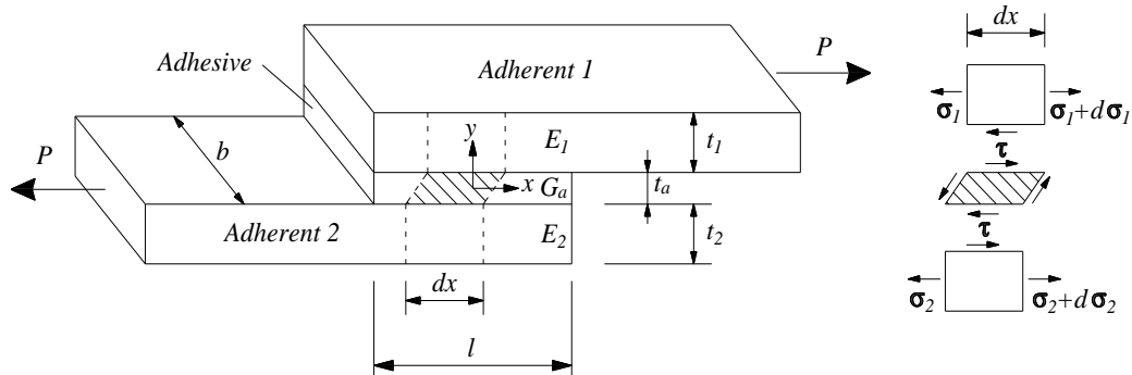
Fig. A 1 Single joint geometry; Volkersen [5].
