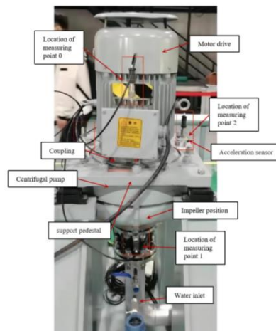
Fig. 9 Schematic diagram of experimental setup
