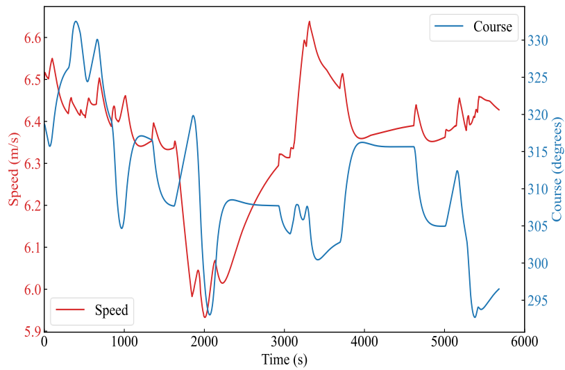
Fig. 22 Simulation experiment of the own-ship (OS) course and speed
