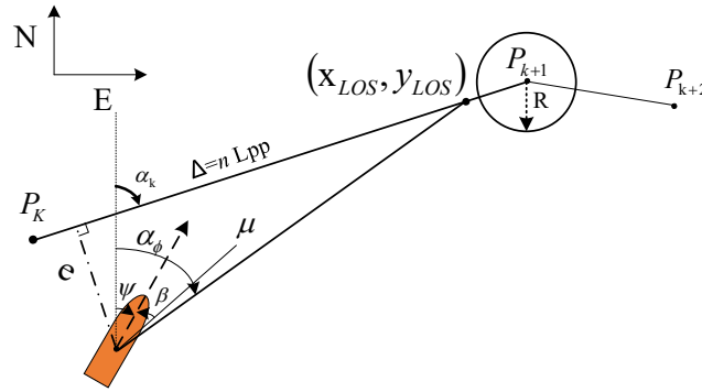
Fig. 14 Schematic of line-of-sight (LOS) guidance
