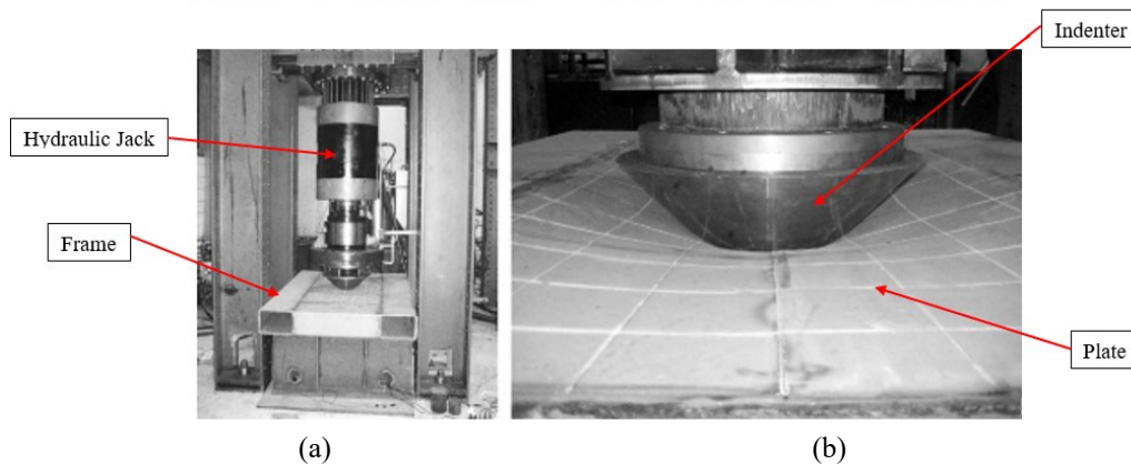
Fig. 3 Alsos et al. [17] experimental test: (a) test setup, and (b) penetration of stiffened plate panel by the indenter
