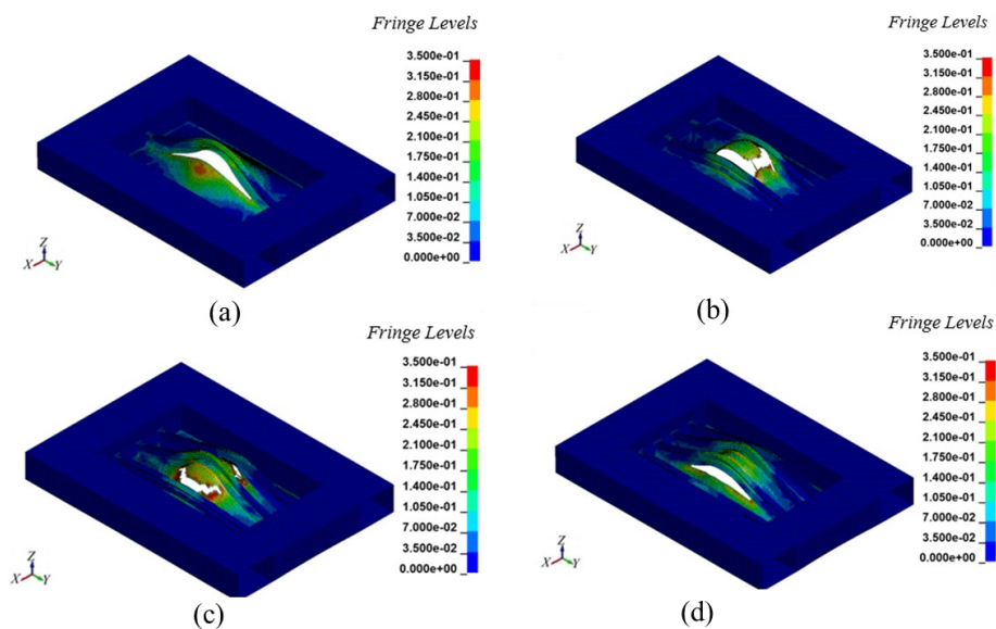
Fig. 21 Effective plastic strain contours at displacement 240 mm: a) Spacing 1, b) Spacing 2, c) Spacing 3, d) Spacing 4
