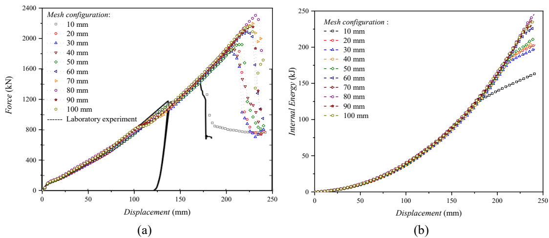
Fig. 14 Simulation result under mesh size variation, a) force-displacement graph, b) internal energy.
