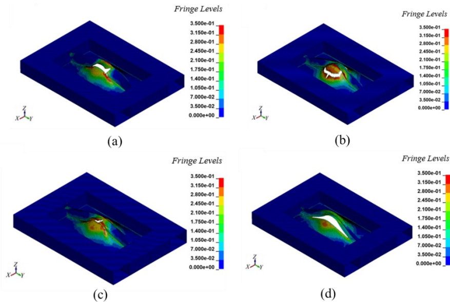
Fig. 18 Effective plastic strain contours at displacement 240 mm: a) Single-I type, b) Single-L type, c) Single-T type, d) Single-Y type
