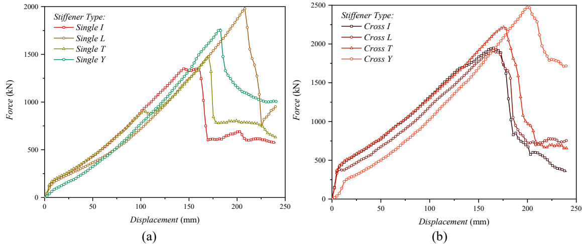
Fig. 16 Force-displacement graph on stiffener type variation: a) single stiffener geometry, a) cross stiffener geometry
