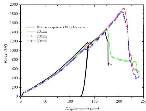
Fig. 5 Force-displacement between numerical and experimental test of single stiffened (1S) structure
