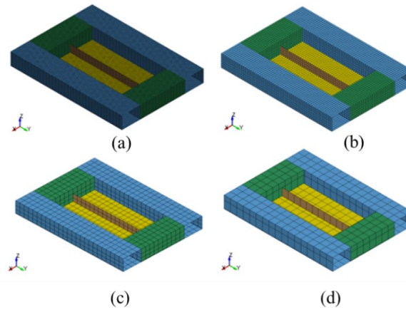
Fig. 9 Mesh size variation geometry: (a) 10 mm, (b) 30 mm, (c) 70 mm, (d) 100 mm
