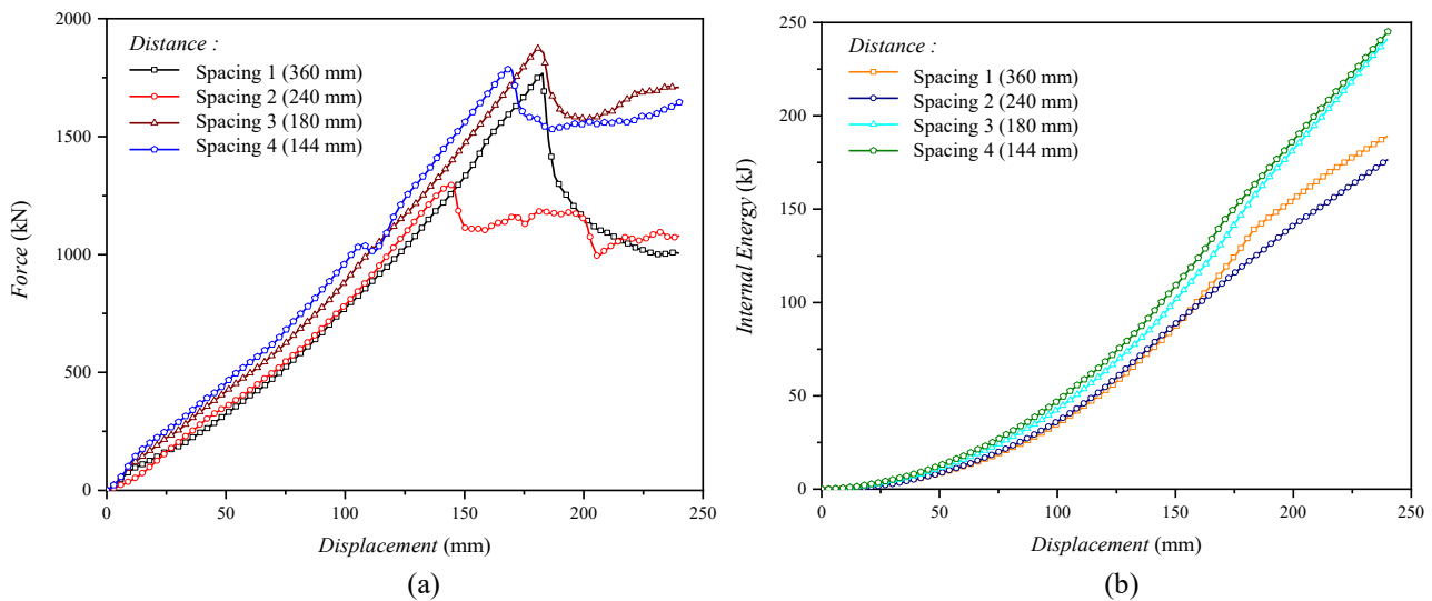
Fig. 20 Simulation result under stiffener spacing variations: a) force-displacement graph, b) internal energy
