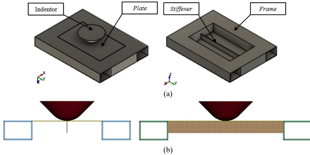
Fig. 7 (a) structural geometries of stiffened plate panel and impactor, (b) shell geometry adjustment
