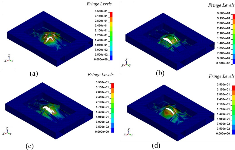
Fig. 23 Effective plastic strain contours at displacement 240 mm: a) Config. 1, b) Config. 2, c) Config. 3, d) Config. 4
