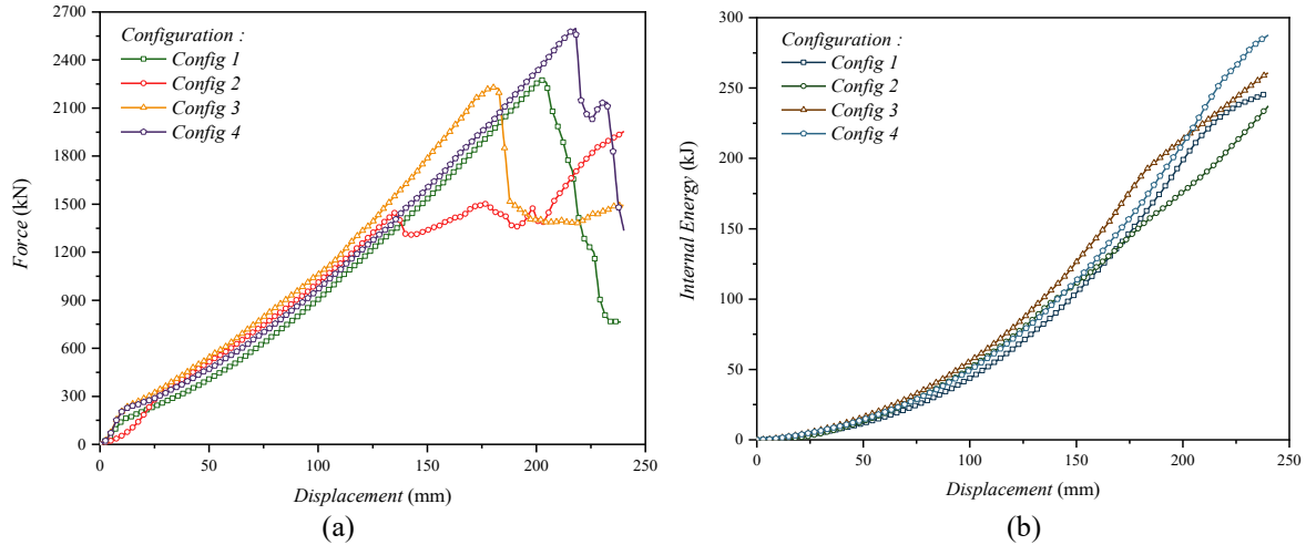
Fig. 22 Simulation result under stiffener configuration variations: a) force-displacement graph, b) internal energy
