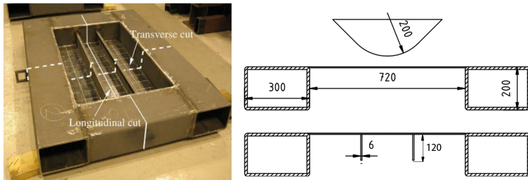
Fig. 1 Structural geometry and dimension of Alsos et al. [17] stiffened plate panel experimental testing
