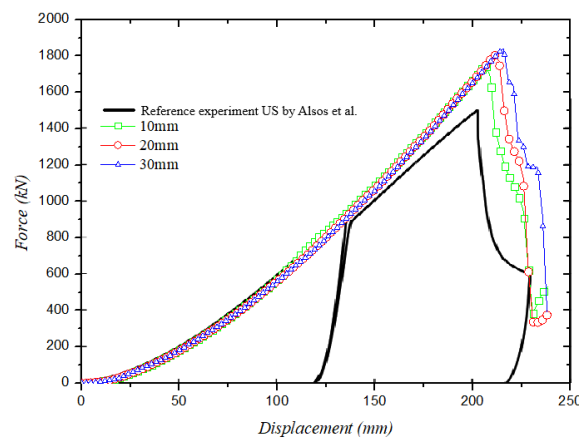
Fig. 4 Force-displacement between numerical and experimental test of unstiffened (US) structure
