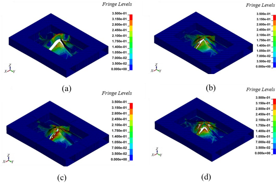
Fig. 19 Effective plastic strain contours at displacement 240 mm: a) Cross-I type, b) Cross-L type, c) Cross-T type, d) Cross-Y type
