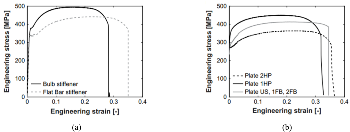
Fig. 2 Material engineering stress-strain curve [17]: (a) stiffener, (b) plate
