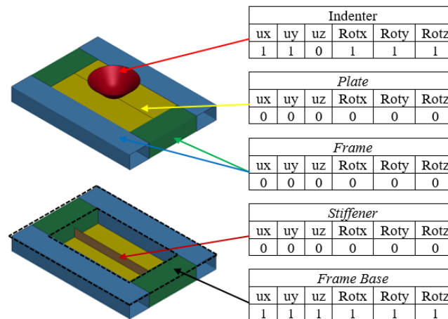
Fig. 8. Schematic loading condition and boundary conditions
