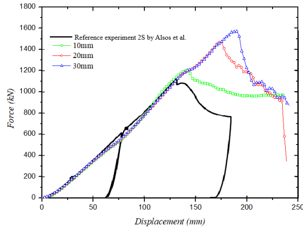
Fig. 6 Force-displacement between numerical and experimental test of double stiffened (2S) structure
