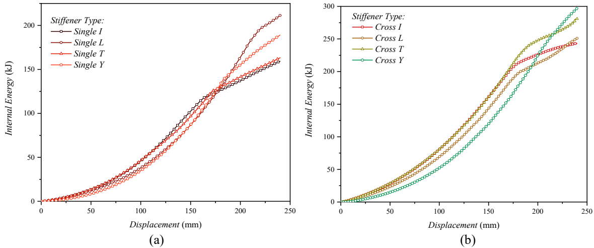
Fig. 17 Internal energy on various stiffener types: (a) single stiffener geometry, (b) cross stiffener geometry
