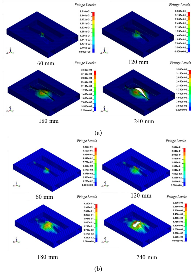
Fig. 15 Effective plastic strain contours at various displacements (a) (a) Mesh size 10 mm, (b) Mesh size 50 mm
