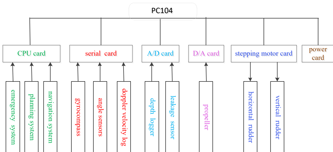
Fig. 2 Hardware architecture of the platform
